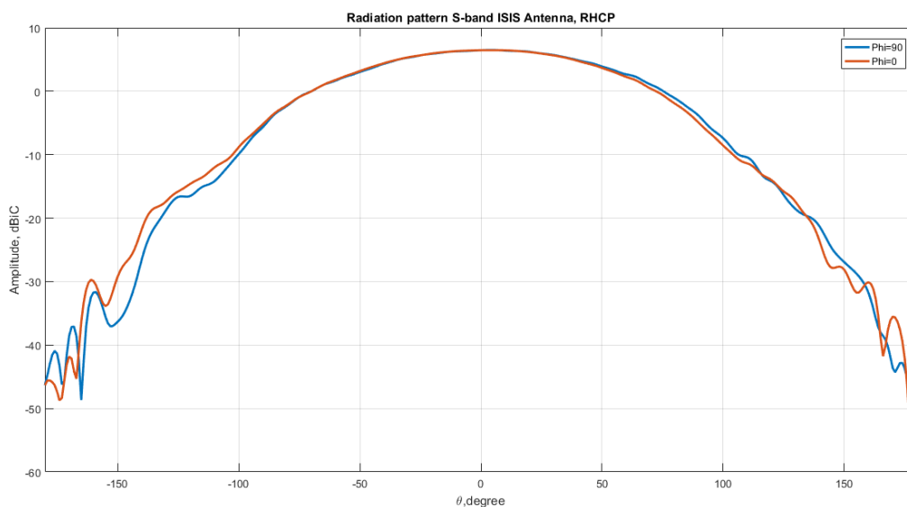
Figure 1 Typical co-polar radiation pattern at 2245 MHz
