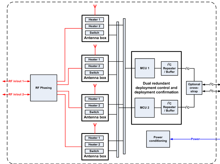
Figure 1 AntS General block diagram
